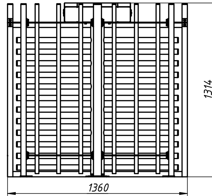
Installation template
