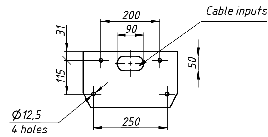
Installation tamplate
