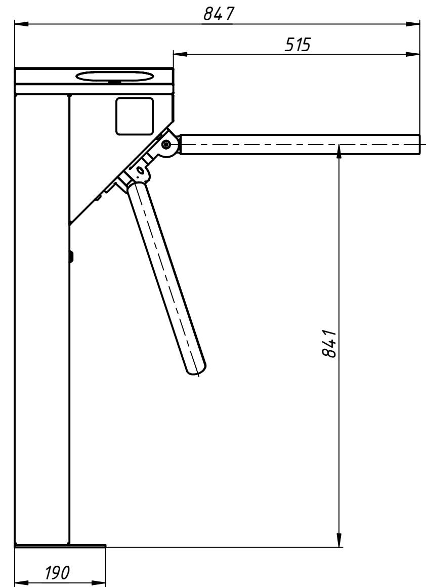
Installation tamplate
